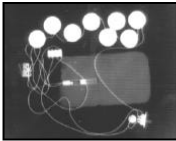
Black and white SCANMAX x-ray image of explosive device
